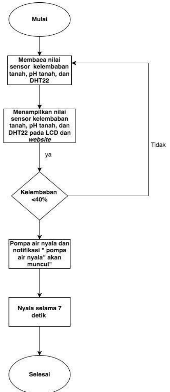
Gambar 11 Flowchart
